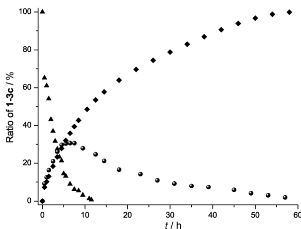
Figure 2. Catalytic formation of indole 2c (●) and 3,3'-biindole 3c (◆) of aniline 1c (▲) in toluene at 70 °C as monitored by 1 H NMR spectroscopy. The residual toluene peak was used as internal standard.
